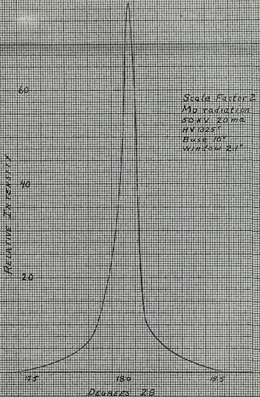
Figure 9. (110)β Peak Brittle Specimen
